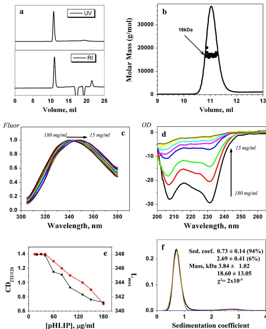
FIGURE 2 pHLP mass in solution at pH 8.0 studied by size-exclusion chromatography coupled with on-line laser light scattering, ultraviolet, and refractive index detection. (a) The UV and RI signals of the major fraction from the column. (b) The results of SEC-LS/UV/RI analysis revealed that the major fraction from the column contained tetrameric pHLP. Normalized fluorescence (c) and CD (d) spectra of various concentrations of pHLP measured in 10 mM phosphate buffer, pH 8.0. The emission spectra were measured at an excitation wavelength of 295 nm. The spectral maximum shifts from 341 to 348 upon dilution. At high peptide concentration, the CD spectra have a characteristic exciton pattern (minimum at 232 nm), which disappears at low concentration where the peptide adopts a random configuration. (e) The pHLP concentration dependence in solution of the fluorescence maximum (red point and line) and the 232:126 nm ratio of the CD signal (black point and line). (f) The distribution of sedimentation coefficients (black line) obtained by analysis of sedimentation velocity runs obtained for 30 \mu\text{g/mL} of pHLP in 10 mM phosphate buffer, 100 mM NaCl, pH 8.0 using the SEDFIT program. The distribution was fitted by Gaussian functions and two components were revealed (the theoretical line is red, the components are green and blue). One predominant component was found, corresponding to a peptide molecular mass of 3.84 kDa (molecular mass of the peptide is 4.1 kDa). Similar results were obtained by applying the SVEDBERG program (see text).
