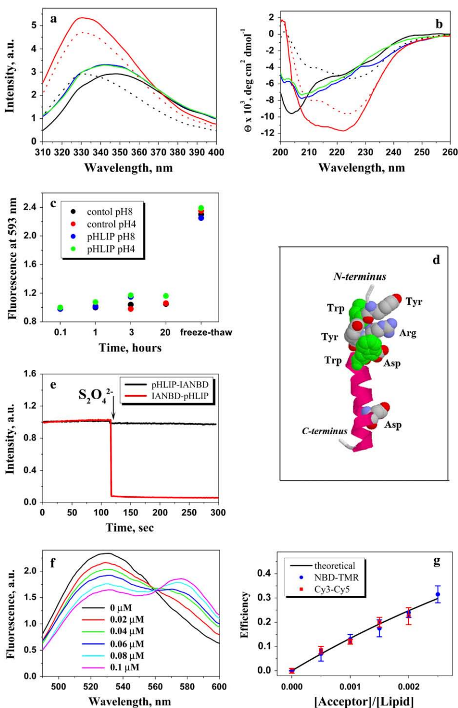
FIGURE 3 Tryptophan fluorescence (a) and CD (b) spectra of 30 \mu g/mL pHLIP in 10 mM phosphate buffer in the absence and presence of POPC liposomes at various pHs. The fluorescence and CD spectra of pHLIP at pH 8.0 (black solid line) indicate a random configuration with tryptophan residues fully exposed to solvent. However, at low pH (pH 3.5) (black dotted line) the peptide tends to aggregate, leading to a shift of position of the fluorescence maximum and the appearance of some elements of secondary structure. Incubation of pHLIP with the POPC liposomes at pH 8.0 (blue solid line) induces the burial of tryptophan residues inside the lipid bilayer without helix formation. Decreasing the pH to 4.0 by the addition of HCl (red solid line) induces the insertion of pHLIP and the formation of helix. When POPC vesicles were added to the pHLIP at pH 3.5 there was an increase of fluorescence, a shift of the spectrum to short wavelengths, and an enhancement of helicity (red dotted line). The insertion of pHLIP across the lipid bilayer is a reversible process; an increase of pH leads to a loss of helicity and the release of the peptide from the membrane (green solid line). (c) The ability of pHLIP to induce vesicle fusion was tested on a mixture of two populations of vesicles with NDB and rhodamine fluorescently-labeled lipids. The graph presents the changes of rhodamine fluorescent signal during incubation of labeled vesicles in the presence of pHLIP at pH 8.0 and 4.0. The values were normalized to the rhodamine fluorescence (at 593 nm, excited at 450 nm) recorded after mixing of NDB-labeled liposomes with rhodamine-labeled liposomes in the absence of pHLIP. A significant increase of emission signal was observed only after several freeze-thaw cycles, which led to the fusion of vesicles. (d) An atomic representation of pHLIP taken from the crystal structure 1C3W (the C helix of bacteriorhodopsin) was generated by RasWin Molecular Graphics 2.6. The green are tryptophan residues. (e) The topology of pHLIP in a lipid bilayer was determined using the IANBD-dithionite quenching reaction. The fluorescence signal of IANBD attached to an SH group at the N-terminus (IANBD-pHLIP) or C-terminus (pHLIP-IANBD) of the peptide was monitored at 550 nm (excited at 478 nm). The starting point is a signal of IANBD-pHLIP and pHLIP-IANBD incubated with POPC followed by lowering the pH to 4.0. Then, dithionite was added. In case of IANBD conjugated to the C-terminus no change of signal is observed (black line), while the fluorescence of IANBD conjugated to the N-terminus of peptide is completely quenched (red line). The data indicate that the N-terminus of pHLIP stays outside, but that the C-terminus of pHLIP goes inside of the vesicles. (f) The pHLIP oligomeric state in a lipid bilayer was studied by FRET. The N-terminus of pHLIP was conjugated either with NDB or TAMRA. Fluorescence spectra of NDB were measured in the presence of an increasing concentration of TAMRA-pHLIP while keeping the total peptide and lipid concentration constant. (g) The comparison of calculated efficiency of energy transfer for NDB-TAMRA (blue points) and Cy3-Cy5 (red points) pairs with the theoretically predicted efficiency of energy transfer (black line) calculated from the Wolber-Hudson equation for noninteracting molecules.
